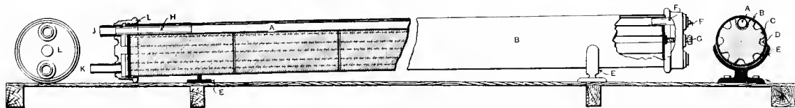
Fig. 3010. GOLD'S TERRA-COTTA STORAGE HEATER.
